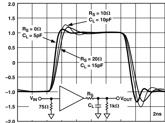
Figure 2. Driving Capacitive Loads
